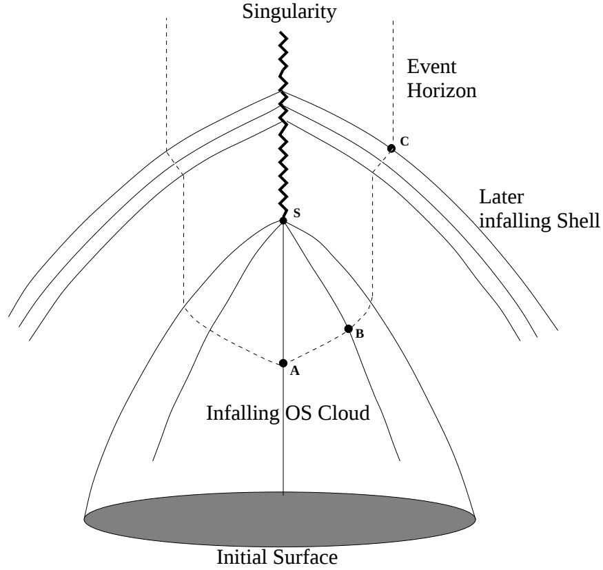
FIG. 1: Gravitational collapse of a spherical pressureless matter cloud (dust cloud) of uniform density whose initial state is shown by the shaded region at the bottom. Time increases in the vertical direction, and space is represented by the horizontal directions. The thin solid lines show worldlines of infalling matter. The event horizon (dashed line) first forms on the worldline of the center of the cloud, at the space-time point A, where conditions are very non-singular. Even point B, on the worldline of matter farther out in the cloud, is at an earlier time than the epoch corresponding to S, where the singularity (thick jagged line) first forms. Although the point C, on a subsequently infalling shell of matter, is at a later time than S, no signals can reach this point from the singularity. Therefore, if any new physics, e.g. firewall or chaos, is to be triggered at A or B or C, it has to be via information traveling back from the future, either along the horizon from future infinity or along worldlines of matter backward from the singularity. This is the teleological paradox, which is caused by the fact that the event horizon is causally cutoff from the singularity, a consequence of cosmic censorship.
