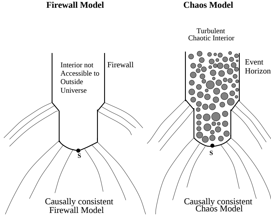
FIG. 3: A causally consistent version of the firewall (left) and chaos (right) models. Both models require some exotic phenomenon — a singular firewall or chaotic dynamics — to switch on suddenly at the horizon (thick solid lines). To trigger this behaviour, a warning of some sort must reach fluid that is about to cross the horizon. Because of cosmic censorship, no such warning from the past is possible if the collapse behaves as in Figure 1. In contrast, when the event horizon connects to the singularity in the past, as in the case of the naked singularity scenario shown in Figure 2, signals from the singularity travel to all points on the horizon. Since the singularity is a region of extreme physical conditions corresponding to the quantum gravity regime, signals originating from here could, in principle, trigger the necessary behaviour for the firewall and chaos models. (No specific trigger mechanism is described here since the focus is on establishing causality.)
