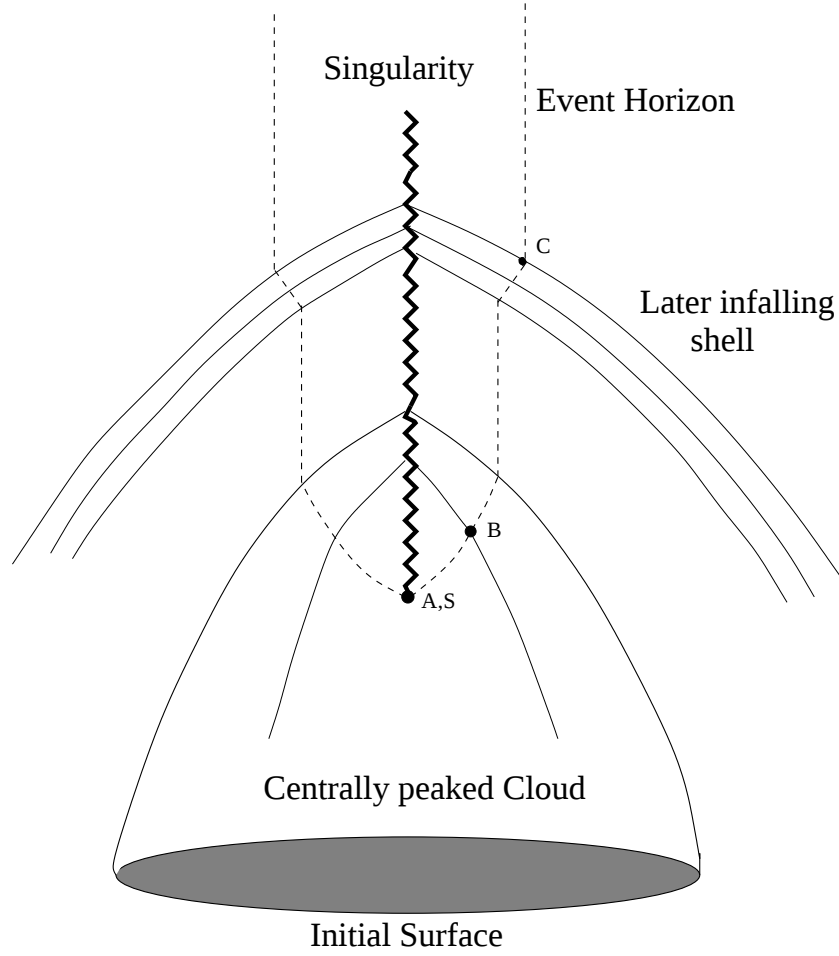
FIG. 2: Gravitational collapse of a spherical dust cloud with a density maximum at the center (equation 2). A naked singularity S forms at A , and the event horizon (dashed line) also originates at A . As a result, the singularity can communicate with the entire event horizon, including points such as B and C . New physics, e.g., firewall or chaos, could thus be triggered on the horizon by signals from S , i.e., from the past. Because of the presence of a naked singularity, this model violates cosmic censorship, which is rather restrictive and is confined to special models such as in Figure 1. Correspondingly, there is no teleological paradox. A wide range of physically reasonable initial conditions of the cloud gives collapse with the causal structure shown here.
